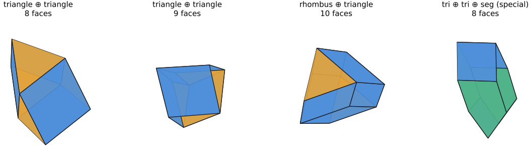
FIGURE 1. Equilateral space-fillers that are Minkowski sums of unit triangles and segments. From left to right: triangle \oplus triangle in the 8-face chamber (generalized gyrobifastigium) and in the 9-face chamber; rhombus \oplus triangle (10 faces); a special position of triangle \oplus triangle \oplus segment (generalized elongated gyrobifastigium, Example 4.6). Triangles are orange, rhombi blue, pentagons green.
