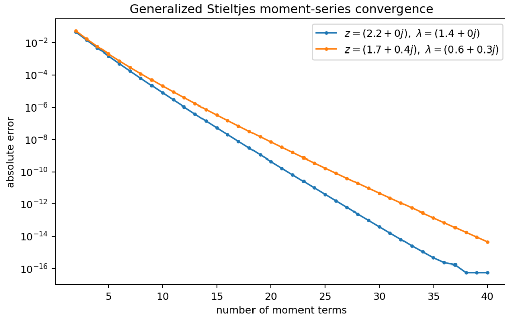
Figure 13: Convergence of the exact-moment expansion (1522) at two real/complex parameter pairs.
