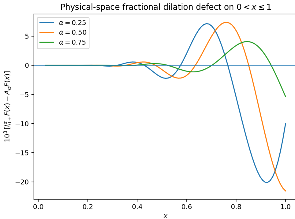
Figure 6: Physical-space comparison of a Riemann–Liouville fractional integral of F with the continuous dyadic interpolation. The visible difference is rescaled; the underlying identity is exact only at integer order.
