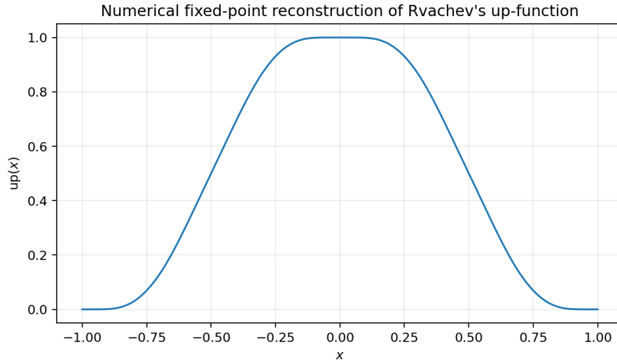
Figure 9: Positive fixed-point reconstruction used for numerical cross-checks. The exact theory, not this discretization, is the source of all theorems.
