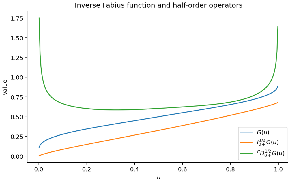
Figure 12: The inverse Fabius function together with its half-order Riemann–Liouville integral and half-order Caputo derivative. The Caputo operator amplifies endpoint structure, whereas the fractional integral smooths it.
