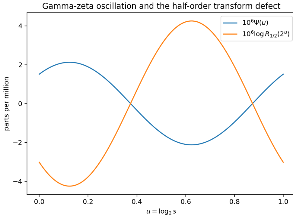
Figure 5: The centered Gamma–zeta oscillation \Psi(u) and the exact half-order defect \log R_{1/2}(2^u) = \Psi(u + 1/2) - \Psi(u) . The vertical scale is in parts per million.
