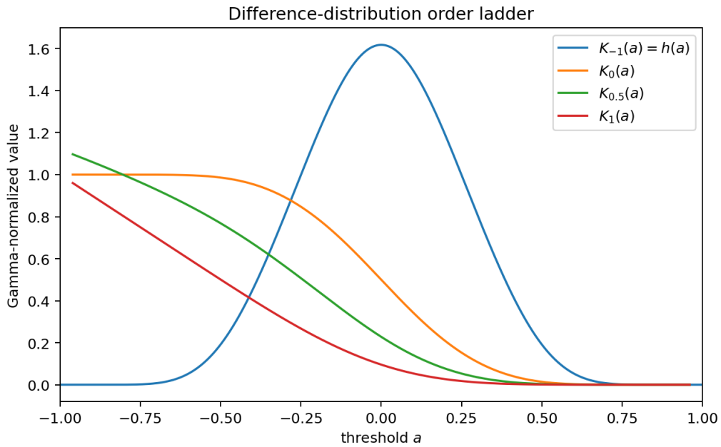
Figure 14: Several real-order slices of the entire difference hierarchy. The order -1 slice is the difference density, order 0 is its tail, and positive orders are fractional positive-part integrals.
