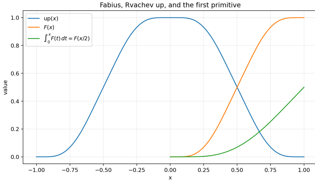
Figure 2: The Fabius function, Rvachev’s up-function, and the exact first primitive \int_0^x F(t) dt = F(x/2) .
