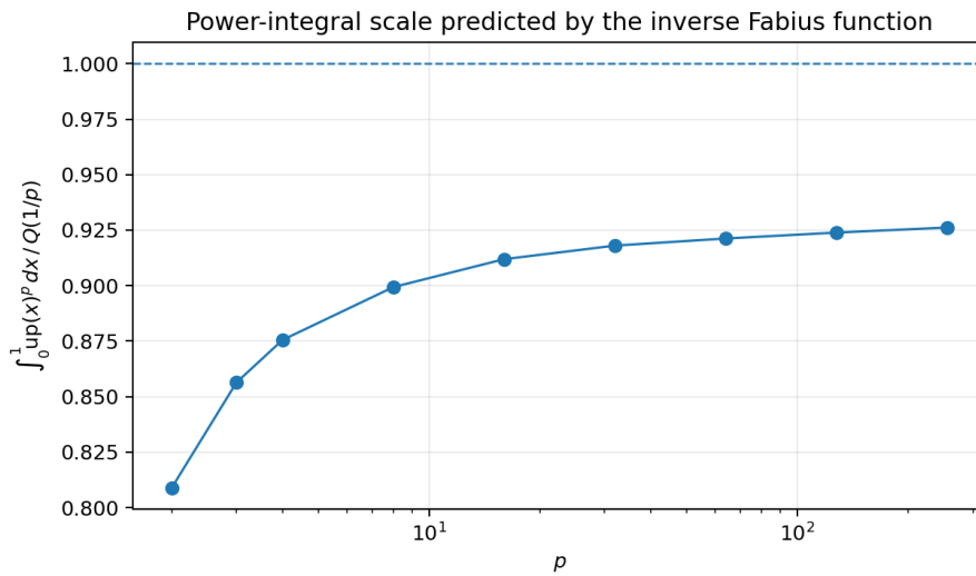
Figure 8: Numerical approach of \int_0^1 \text{up}(x)^p dx / Q(1/p) toward the rigorous limit one. The slow approach reflects the lower-Lambert endpoint scale.
