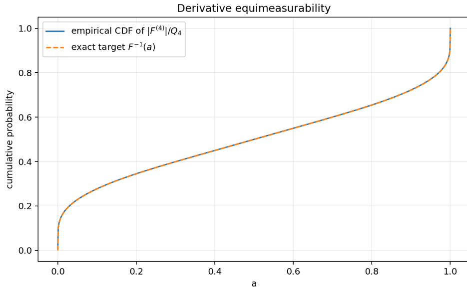
Figure 3: The empirical CDF of |F^{(4)}|/Q_4 lies on the exact target I = F^{-1} , illustrating theorem 9.1 .
