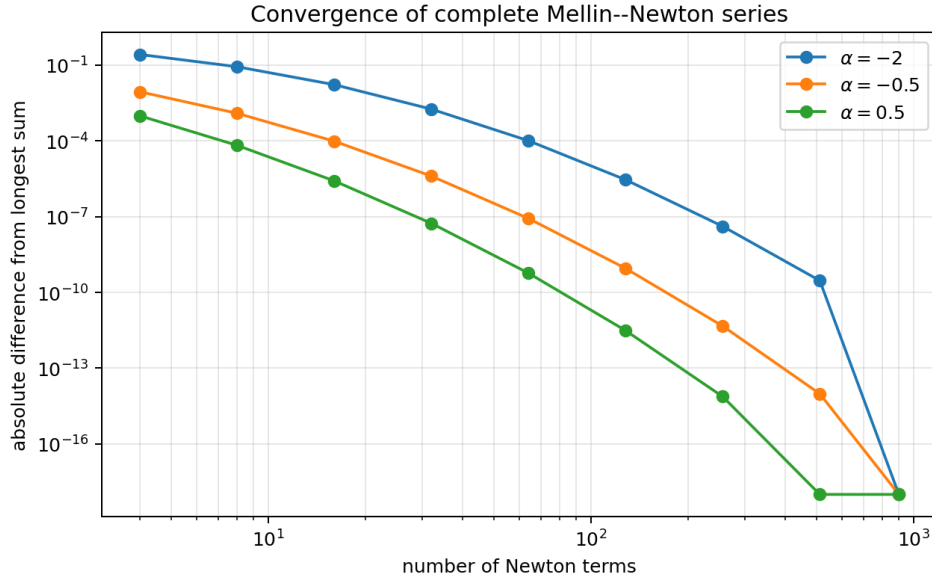
Figure 1: Convergence of the complete Mellin–Newton series. The reference is the longest available 900-term sum, so the final plotted error is clipped at machine scale rather than being a certified remainder.
