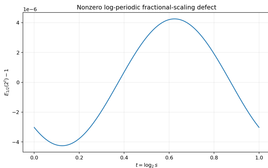
Figure 4: One logarithmic period of the nonzero defect P(t - 1/2)/P(t) - 1 . Its parts-per-million size makes the false fractional scaling law numerically seductive.
