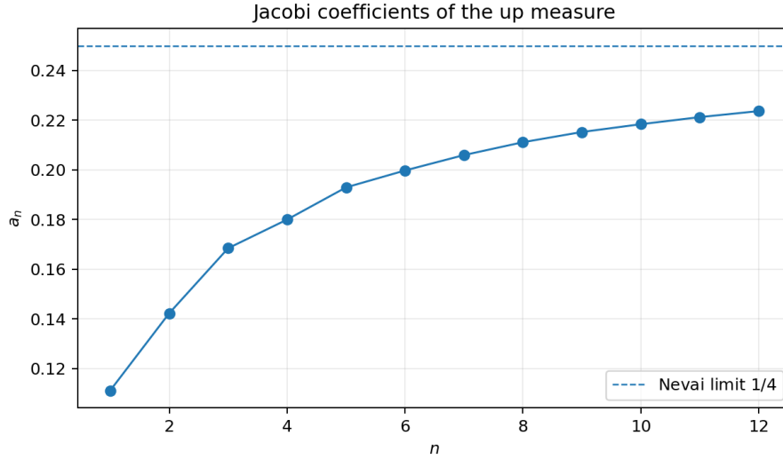
Figure 7: The first twelve exact Jacobi coefficients (shown in decimal form) and the rigorous limiting value 1/4 . Monotonicity is suggested but not proved.
