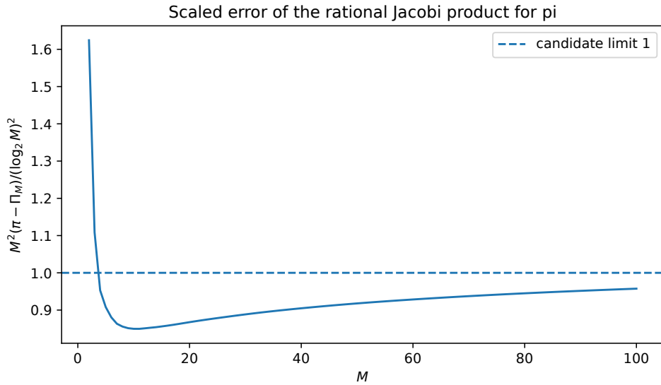
Figure 5: Scaled error of the rational product. The candidate limit 1 is part of theorem 11.2 .
