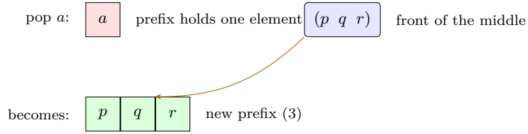
Figure 3: Pull repair, the dual of Figure 2. Popping the sole element of a one-element prefix pulls the front node (p, q, r) up out of the middle and unpacks it into a fresh three-element prefix; only the (rare) underflow descends into the middle.
