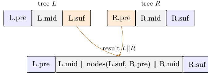
Figure 4: Concatenation. The outer prefix and suffix are inherited from L and R ; the adjacent inner digits (L.suf and R.pre) are regrouped into nodes and merged into a single recursive concatenation of the middles. Here “ \parallel ” denotes sequence concatenation one level down.
