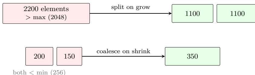
Figure 2: The rope chunk-size policy keeps leaves healthy. An insert that grows a chunk past the maximum splits it (top); adjacent chunks that fall below the minimum coalesce (bottom), including across a concatenation boundary. Healthy chunks bound both the per-edit copy and the tree depth.
