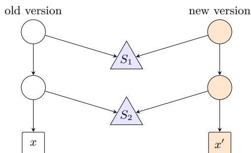
Figure 3: Path copying. Editing leaf x \rightarrow x' allocates only the \mathcal{O}(\log n) nodes on the root-to-leaf path (orange); every off-path subtree ( S_1 , S_2 ) is shared by both versions. The old version is untouched and remains valid — this is why a snapshot is free and an edit is logarithmic.
