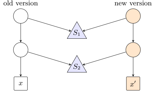
Figure 6: Path copying. Editing leaf x \rightarrow x' allocates only the \mathcal{O}(\log n) nodes on the root-to-leaf path (orange); every off-path subtree ( S_1 , S_2 ) is shared by both versions. The old version is untouched and remains valid — this is why a snapshot is free and an edit is logarithmic.
