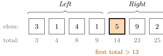
Figure 7: A monotone-predicate split with a sum measure: each cell’s running total is shown beneath it. For the predicate “total > 13”, Split returns the prefix Left and suffix Right ; TrySplitFind also returns the boundary element (highlighted).
