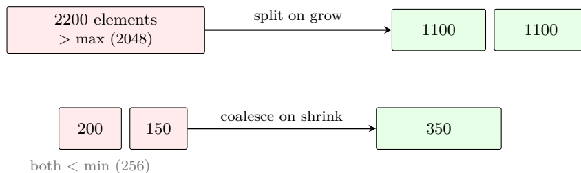
Figure 5: The rope chunk-size policy keeps leaves healthy. An insert that grows a chunk past the maximum splits it (top); adjacent chunks that fall below the minimum coalesce (bottom), including across a concatenation boundary. Healthy chunks bound both the per-edit copy and the tree depth.
