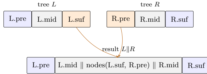
Figure 3: Concatenation. The outer prefix and suffix are inherited from L and R ; the adjacent inner digits (L.suf and R.pre) are regrouped into nodes and merged into a single recursive concatenation of the middles. Here “ \parallel ” denotes sequence concatenation one level down.
