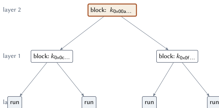
Figure 20.1: Layer assignment in a Merkle search tree. A key’s layer is the number of leading zero nibbles of its SHA-256 digest; one block holds each consecutive same-layer run, and that block’s digest covers the policy domain, its entries, its subtree count, and its child digests. Because the shape comes from the hashes, two processes that insert the same entries in different orders build the same tree and compute the same root digest.
