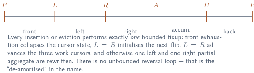
Figure 14.1: The DABA Lite cursor state. The schedule is what makes the operation bounds worst-case rather than amortised.
