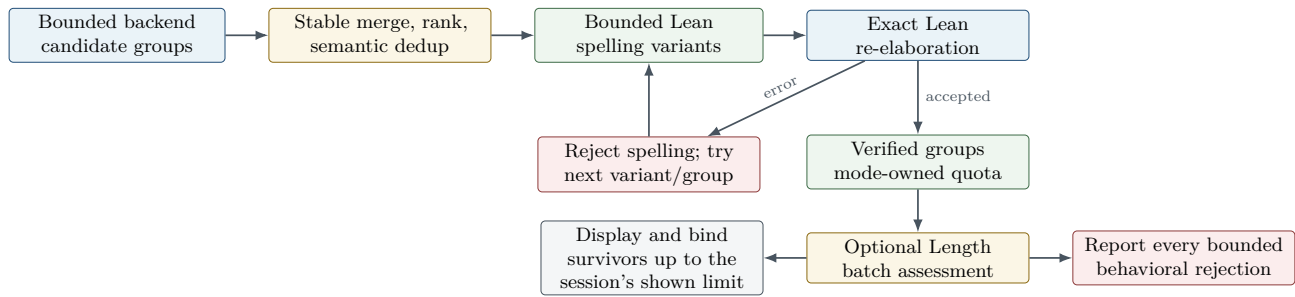
Figure 16.1: The candidate funnel. The exact Lean target remains the acceptance gate; optional behavioral filtering partitions each bounded cursor batch, with at most one successor, before the presentation cap of synth-shown survivors (five by default).
