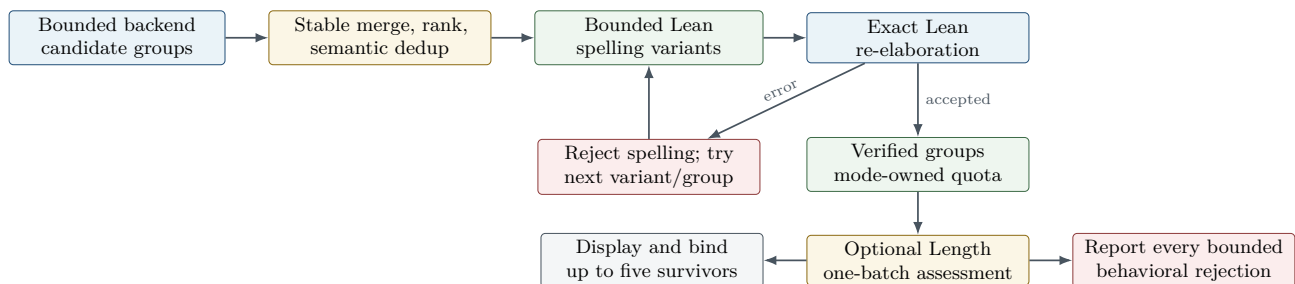
Figure 16.1: The candidate funnel. The exact Lean target remains the acceptance gate; optional behavioral filtering partitions one bounded lane before the five-survivor presentation cap.
