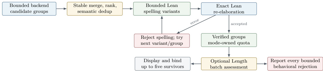
Figure 16.1: The candidate funnel. The exact Lean target remains the acceptance gate; optional behavioral filtering partitions each bounded cursor batch, with at most one successor, before the five-survivor presentation cap.
