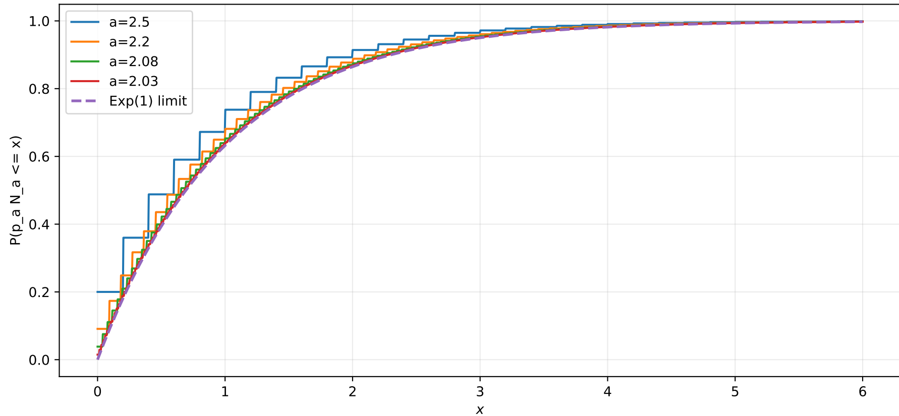
Critical exponential limit of the local polynomial degree
