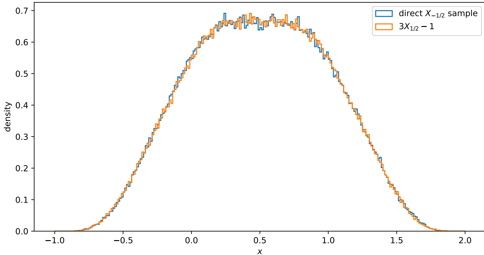
Negative dyadic law: direct and affine-transformed samples
