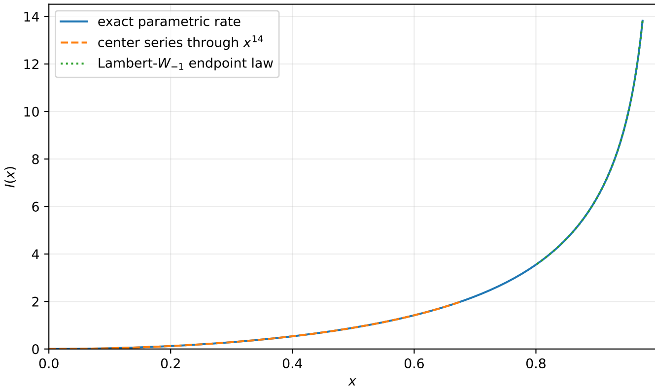
Large-deviation rate function for the geometric-uniform family
