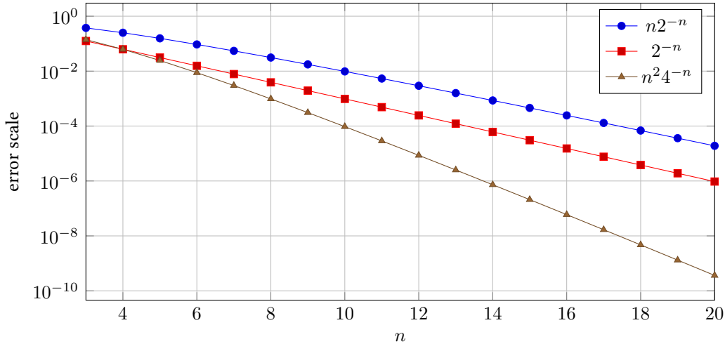
Figure 4: The three scales in (706). The deterministic center drift n2^{-n} dominates the one-cell scale 2^{-n} and the quadratic Taylor scale n^24^{-n} .
