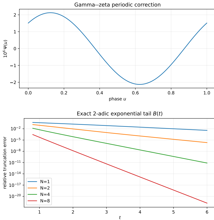
Figure 2: Top: the centered Gamma-zeta fluctuation \Psi – tiny amplitude, same asymptotic order as the constants. Bottom: relative error of N = 1, 2, 4, 8 terms of the exact 2-adic series for B(t) , with the elementary enclosure of theorem 9.2 .
