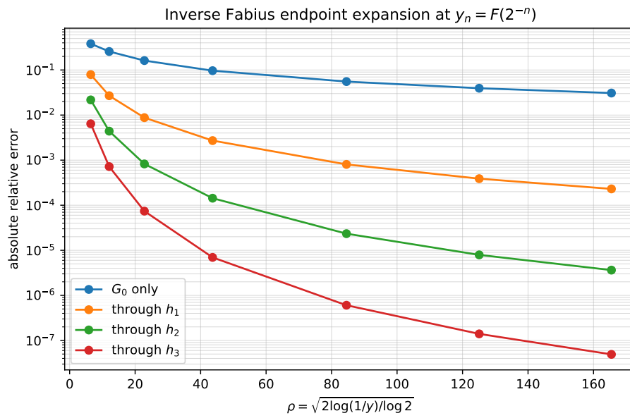
Figure 1: Absolute relative errors on the exact dyadic quantiles; each added logarithmic correction produces the expected strong reduction once \rho is moderately large.
