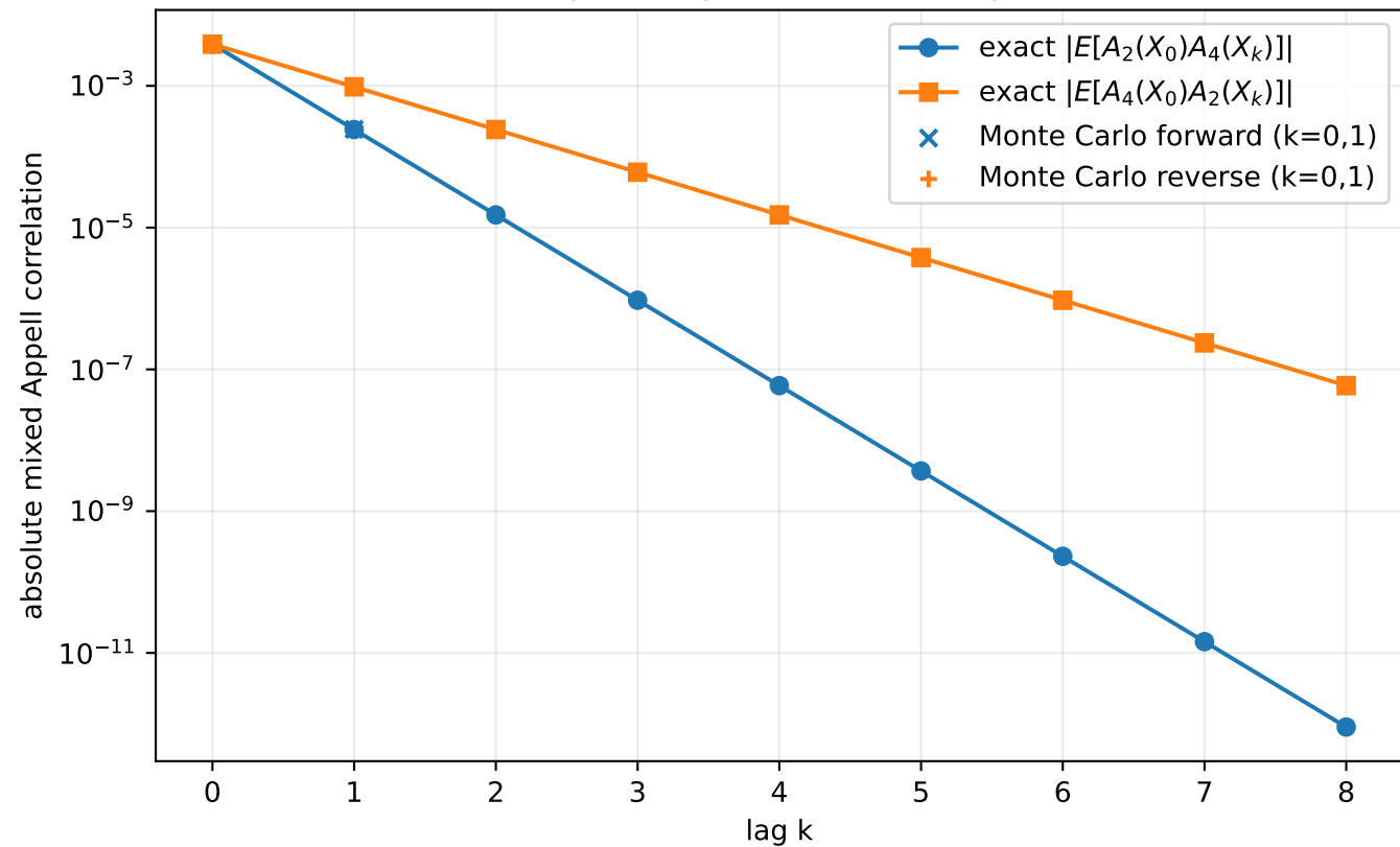
Exact time asymmetry of the stationary affine chain
