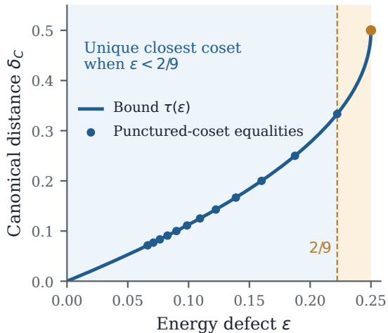
A. Sharp coset envelope
