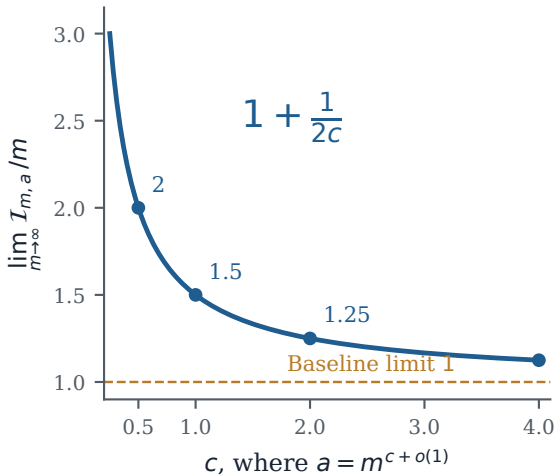
B. Joint arity-order limit
