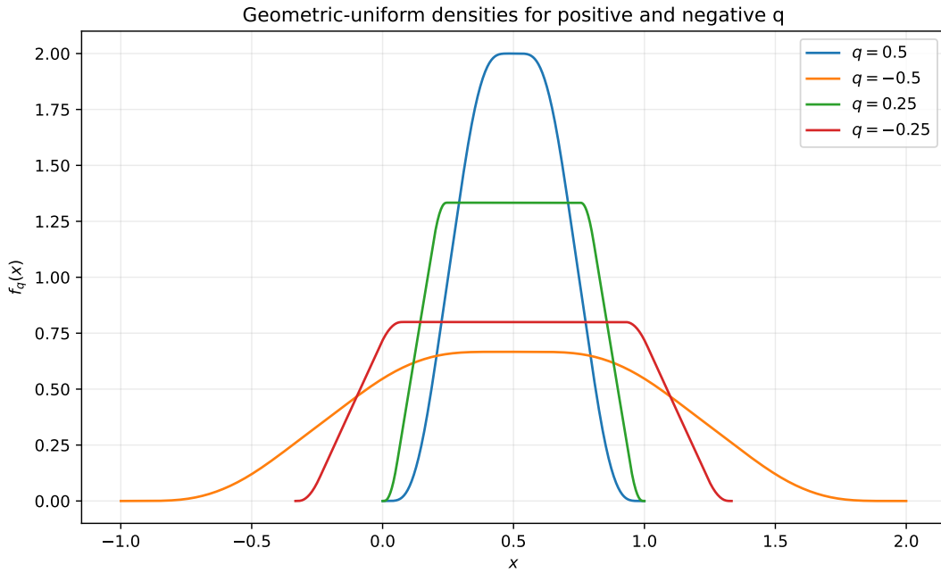
Figure 28: Physical densities for q = \pm\frac{1}{2}, \pm\frac{1}{4} (sixteenth-wave package). The negative curves are exact affine stretches of their positive partners; the quarter-base profiles carry positive-length plateaus, while the half-base plateau is critical and collapses to the center (theorem 4.2).
