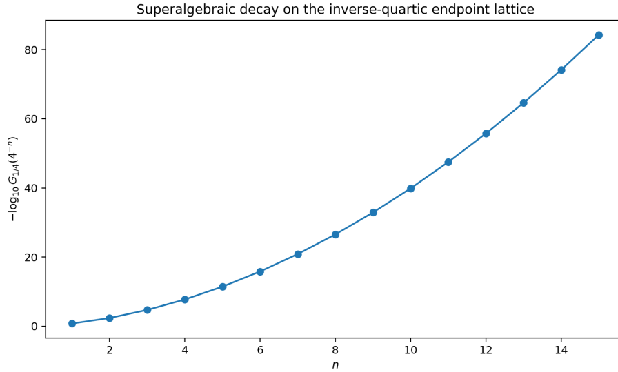
Figure 30: Exact inverse-quartic lattice values (14.3) on a logarithmic ordinate. The quadratic growth of -\log G_{1/4}(4^{-n}) is the discrete shadow of the two-term endpoint law of theorem 15.1.
