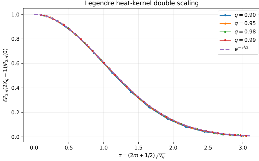
Figure 6: High-precision moment evaluation of the Legendre double scaling. At q = 0.99 the largest absolute discrepancy over the plotted range is about 1.26 \times 10^{-3} .
