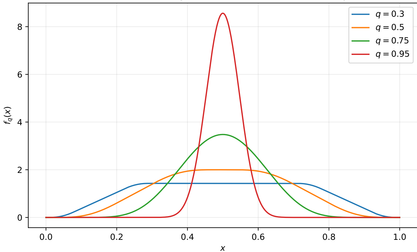
Densities in the geometric Fabius--Rvachev family
