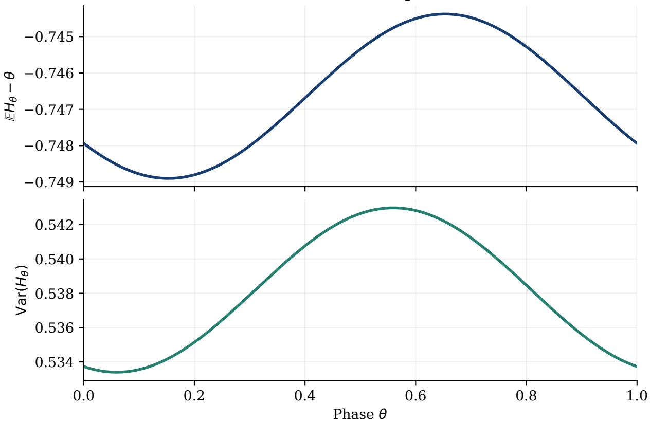
Periodic corrections to the largest Catalan index
