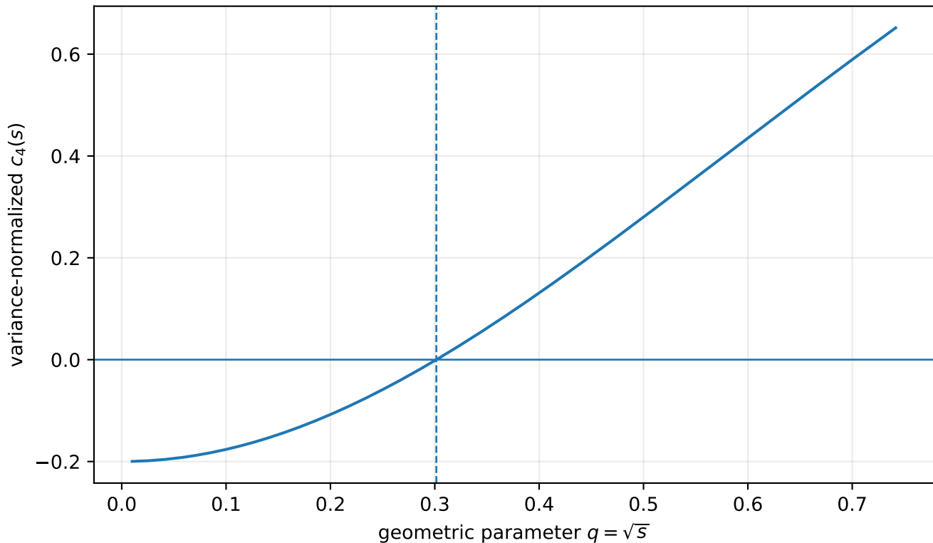
First free-cumulant obstruction in the geometric-uniform family
