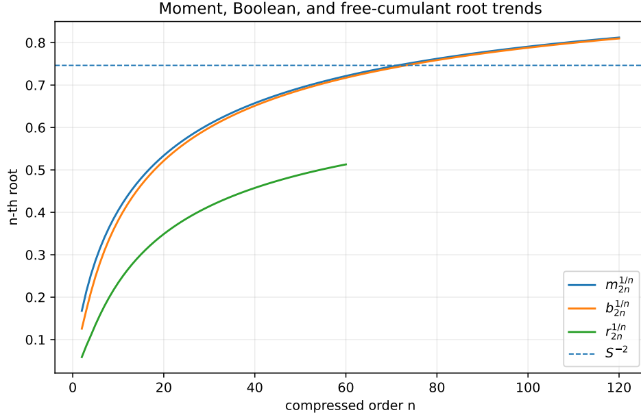
Figure 2: Root diagnostics. The moment and Boolean roots tend slowly to one, while the free-cumulant roots appear to approach the horizontal value S^{-2} . The observed convergence is too slow to be treated as proof.
