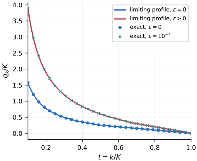
Backward trajectories
