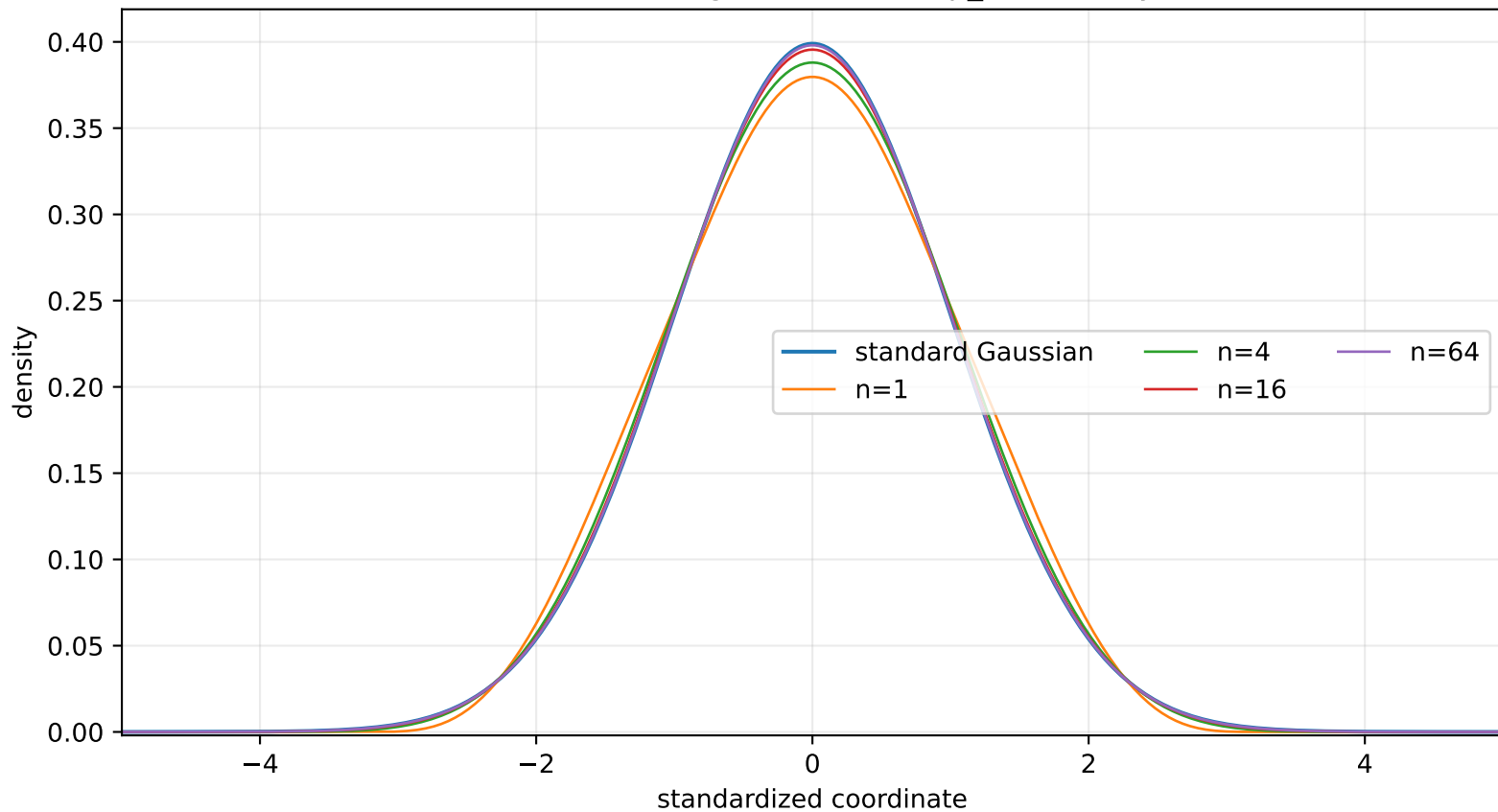
Gaussian scaling limit of the Fup_n hierarchy
