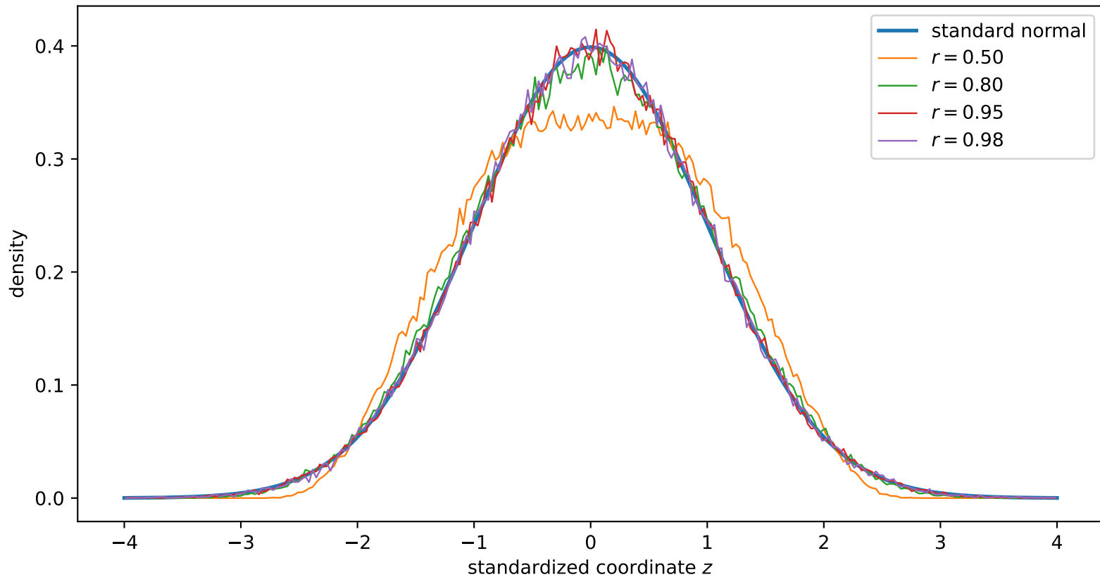
Gaussian boundary for Z_r = (X_r - 1/2)/\sigma_r
