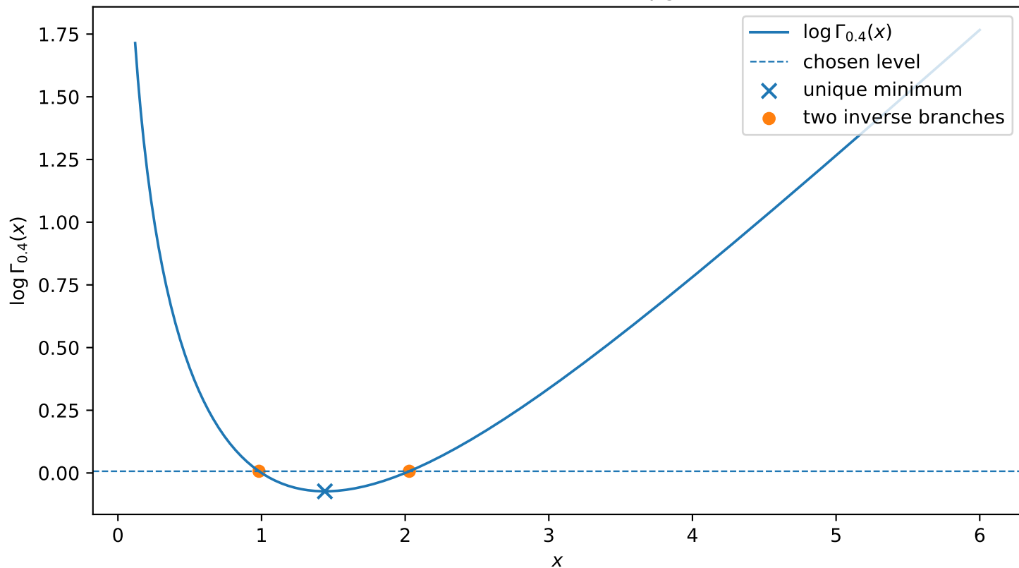
Two real branches of the inverse q-gamma function
