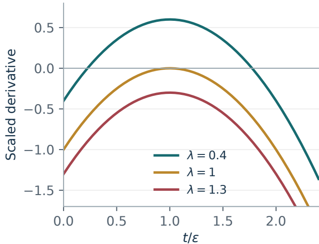
Two roots merge at the fold
