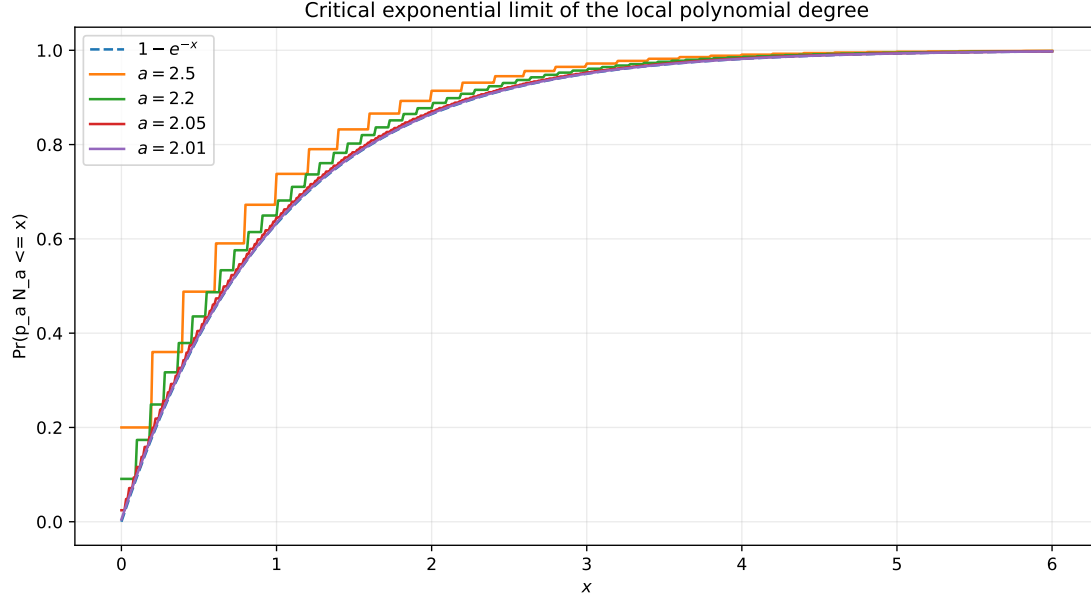
Figure 22: Distribution functions of p_a N_a approaching 1 - e^{-x} as a \downarrow 2 (theorem 13.3).
