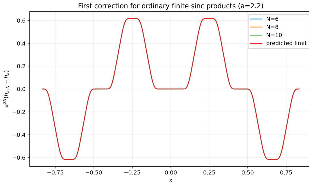
Figure 24: For a = 2.2 , the scaled errors a^{2N}(h_{a,N} - h_a) for N = 6, 8, 10 are visually indistinguishable from -h_a''/[6(a^2 - 1)] . The computation uses FFT inversion of the explicit products, not random sampling.
