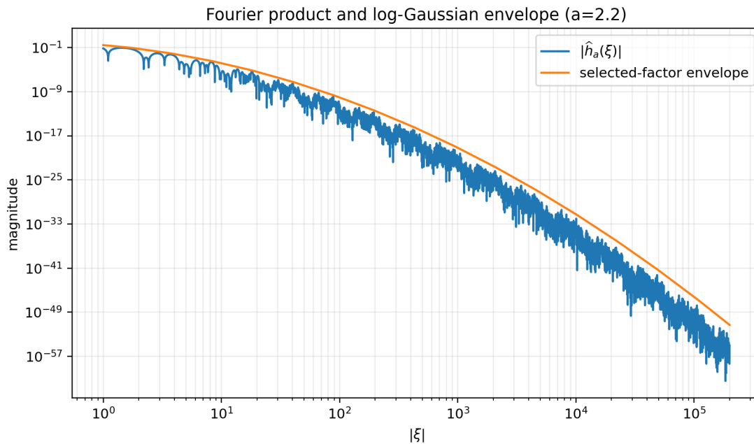
Figure 23: The Fourier product for a = 2.2 and the selected-factor bound (15.1). The oscillatory zeros sit well below the envelope, while the quadratic decay in \log |\xi| is clearly visible.
