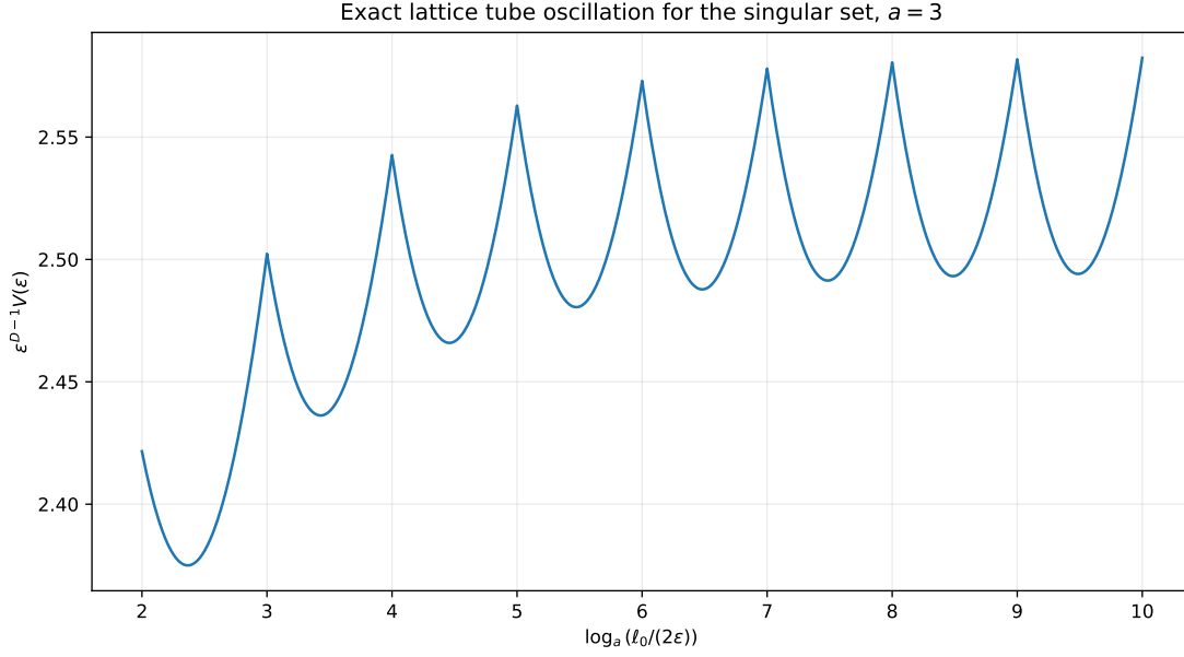
Figure 21: The exact normalized tube volume for a = 3 . The approach to a nonconstant one-periodic profile in \log_a(1/\varepsilon) verifies the lattice oscillation of theorem 13.2 .
