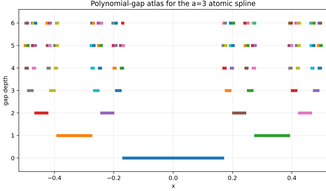
Figure 20: The first seven levels of the gap decomposition for a = 3 . The depth r gaps are the intervals on which the local polynomial degree is exactly r . Their union has full measure in the support [-1/2, 1/2] .
