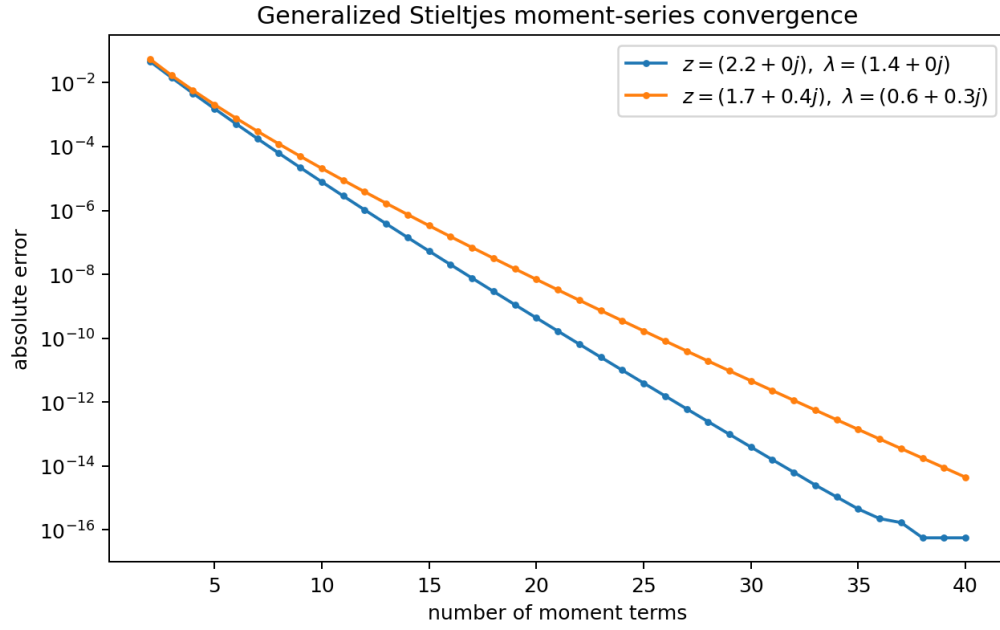
Figure 12: Convergence of the exact-moment expansion (1513) at two real/complex parameter pairs.
