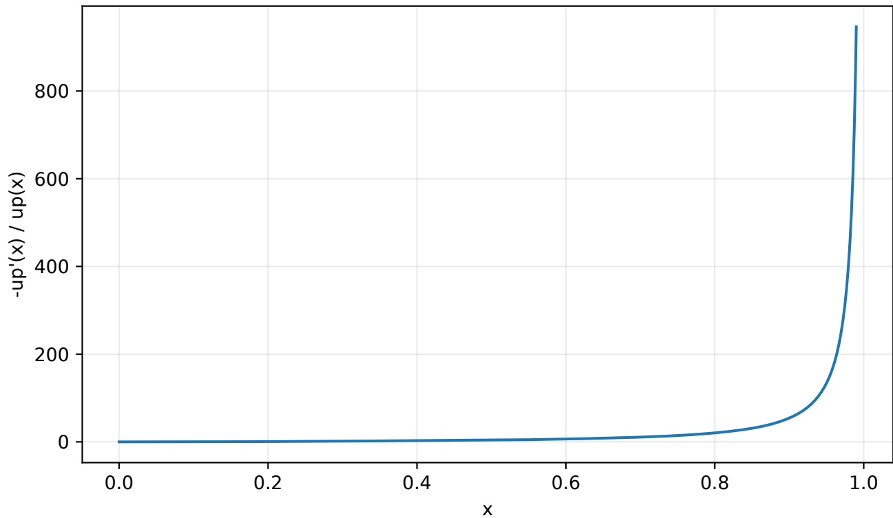
Increasing score predicted by strict log-concavity
