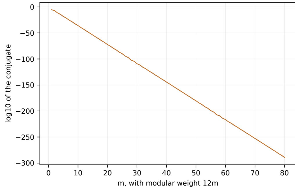
The conjugate from the exact norm law
