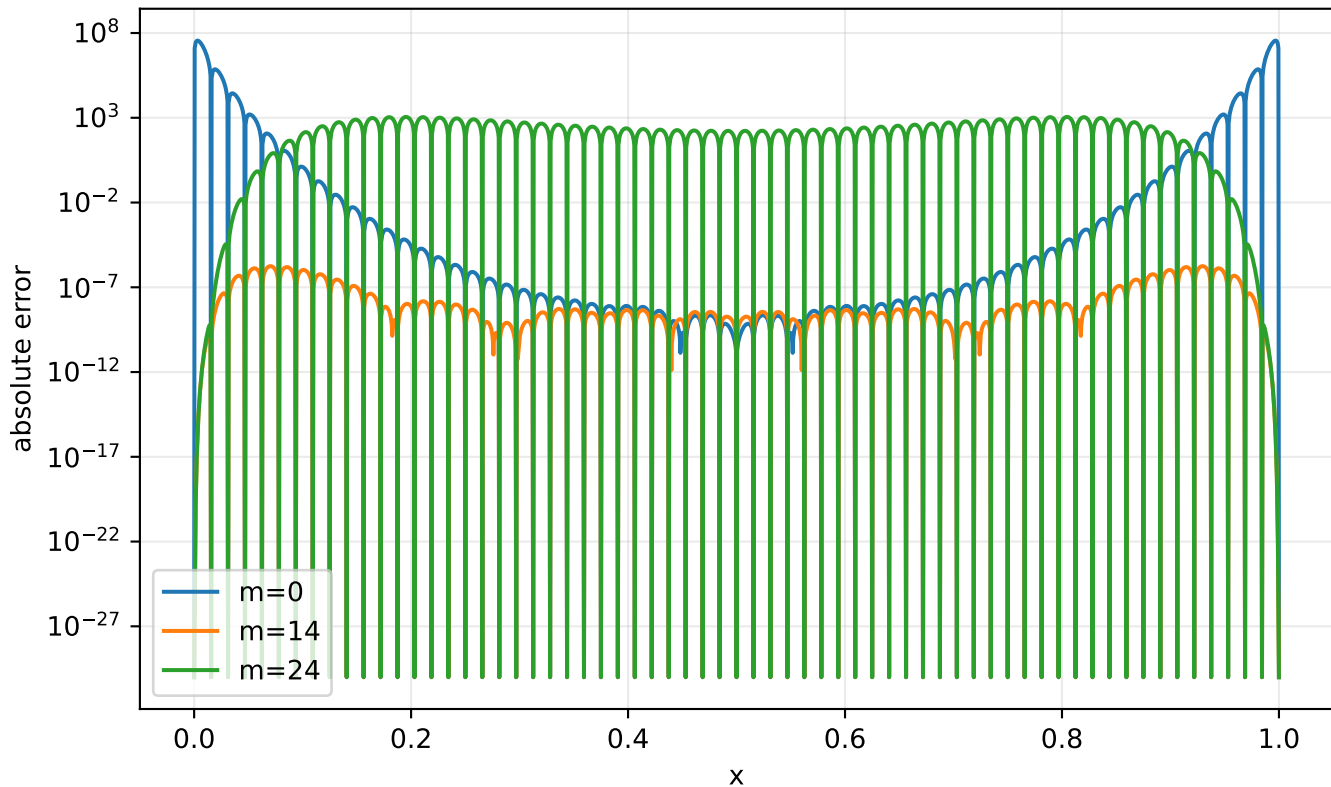
Fabius error profile at N=64
