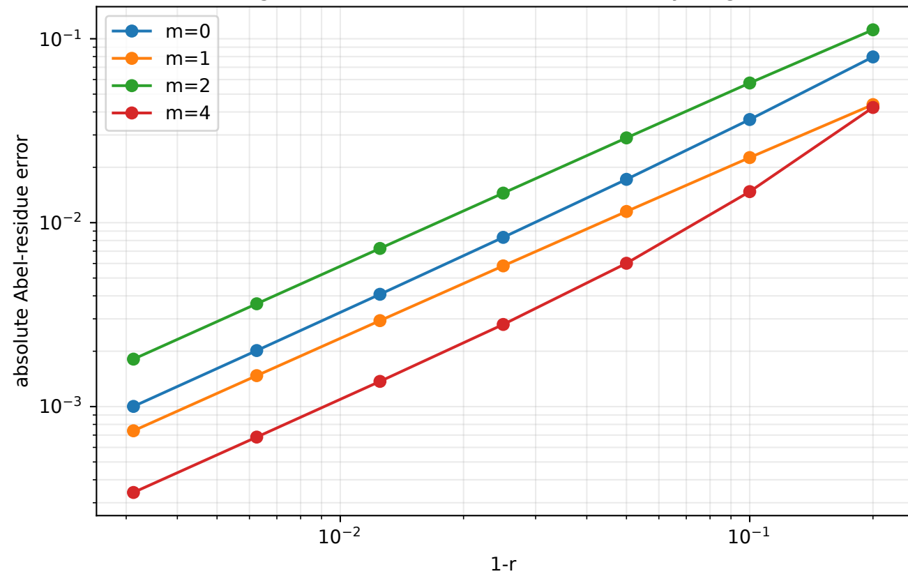
Convergence to Fourier residues at boundary singularities
