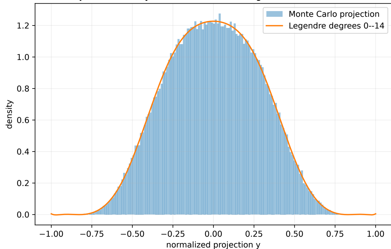
Projection density and Bell--Bernoulli Legendre reconstruction
