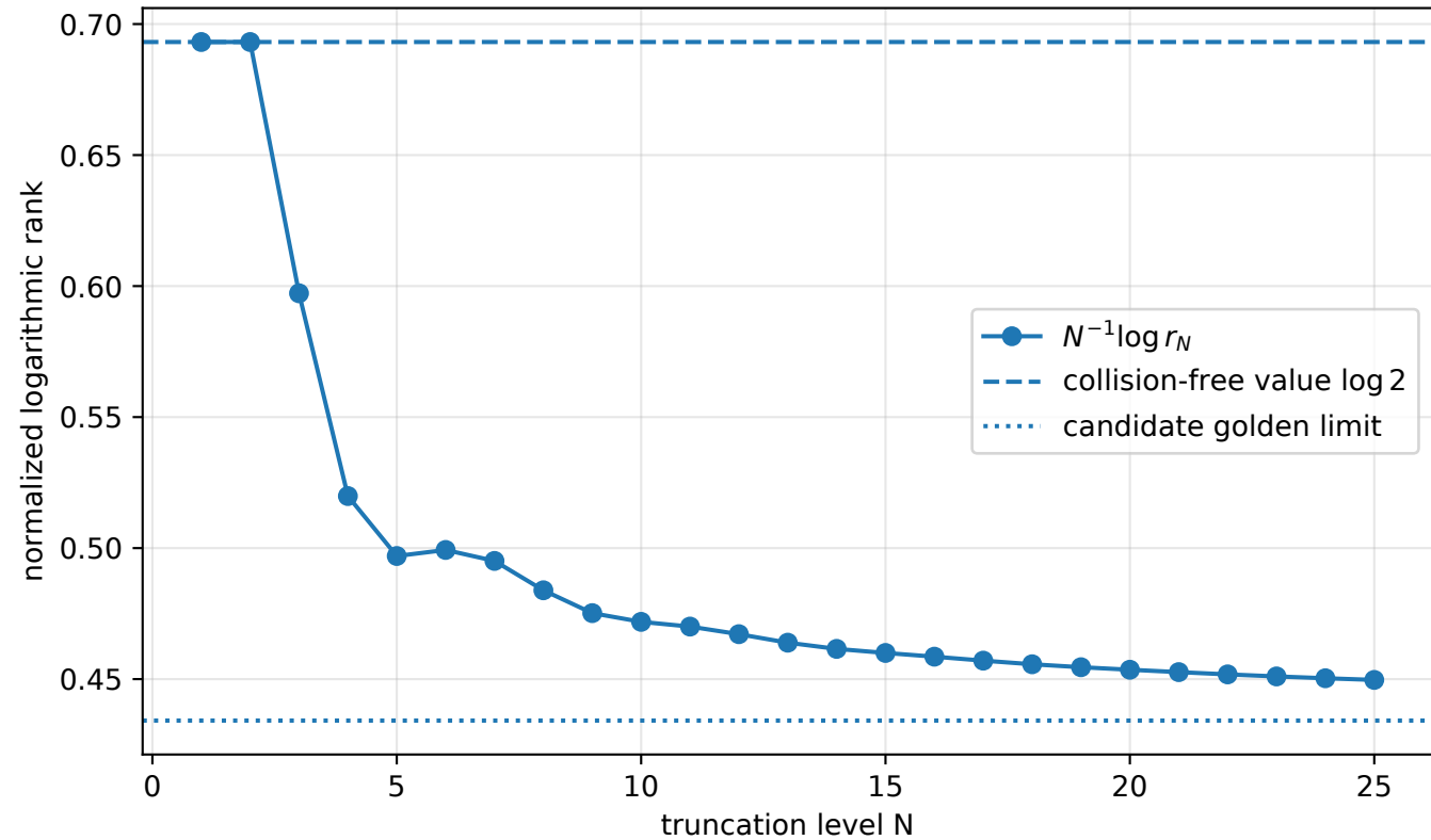
Golden-overlap holonomic entropy
