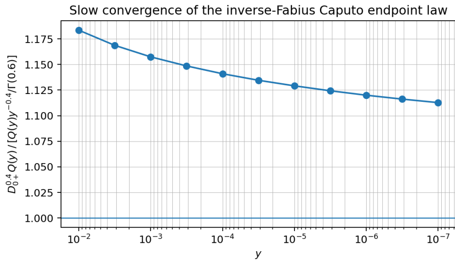
Figure 9: The ratio in equation (1132) for r = 1 and \beta = 0.4 . The theorem predicts convergence to 1; the slow drift exposes the scale of the first Lambert-type correction.
