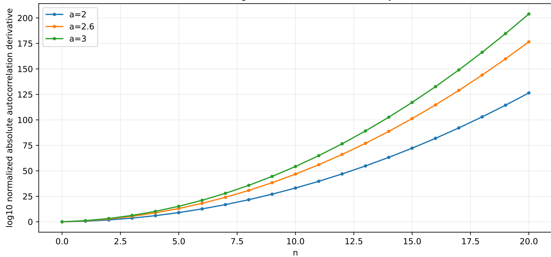
Quadratic growth of the autocorrelation jet
