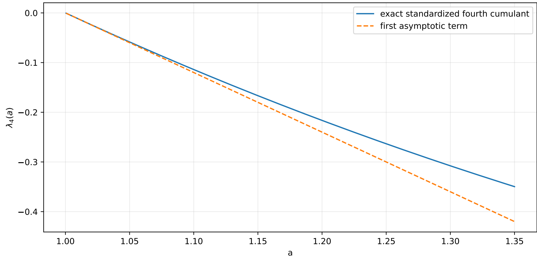
Gaussian cumulant scaling as a \downarrow 1
