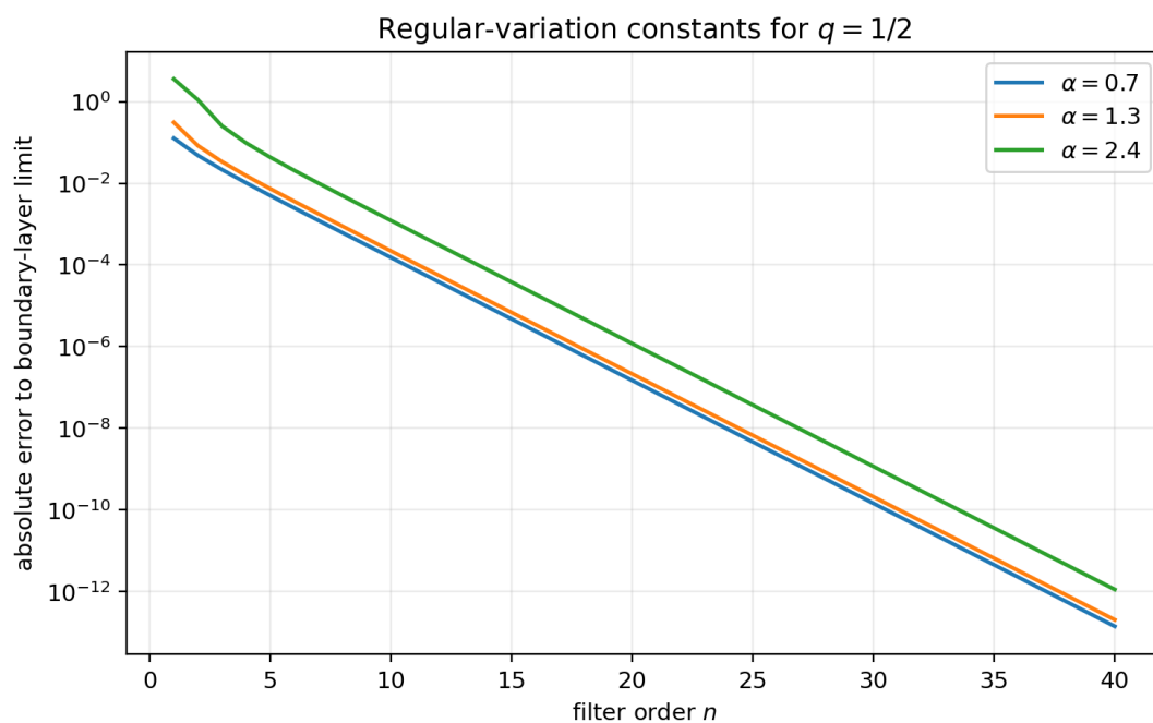
Figure 2: For pure powers x^{\alpha} at q = 1/2 , the normalized exact multiplier (q^{1-\alpha}; q)_n/(q; q)_n converges geometrically to C_q(\alpha) . The three exponents illustrate positive and negative limiting constants.
