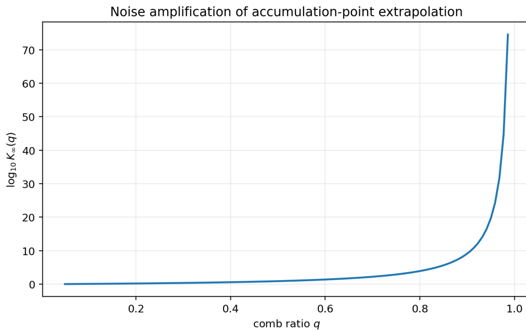
Figure 1: The infinite-order total variation K_{\infty}(q) = (-q; q)_{\infty}/(q; q)_{\infty} . The vertical axis is logarithmic in base 10. Stability is excellent for small and moderate q but deteriorates nonperturbatively as q \uparrow 1 .
