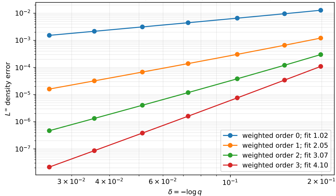
Continuous-parameter Edgeworth hierarchy
