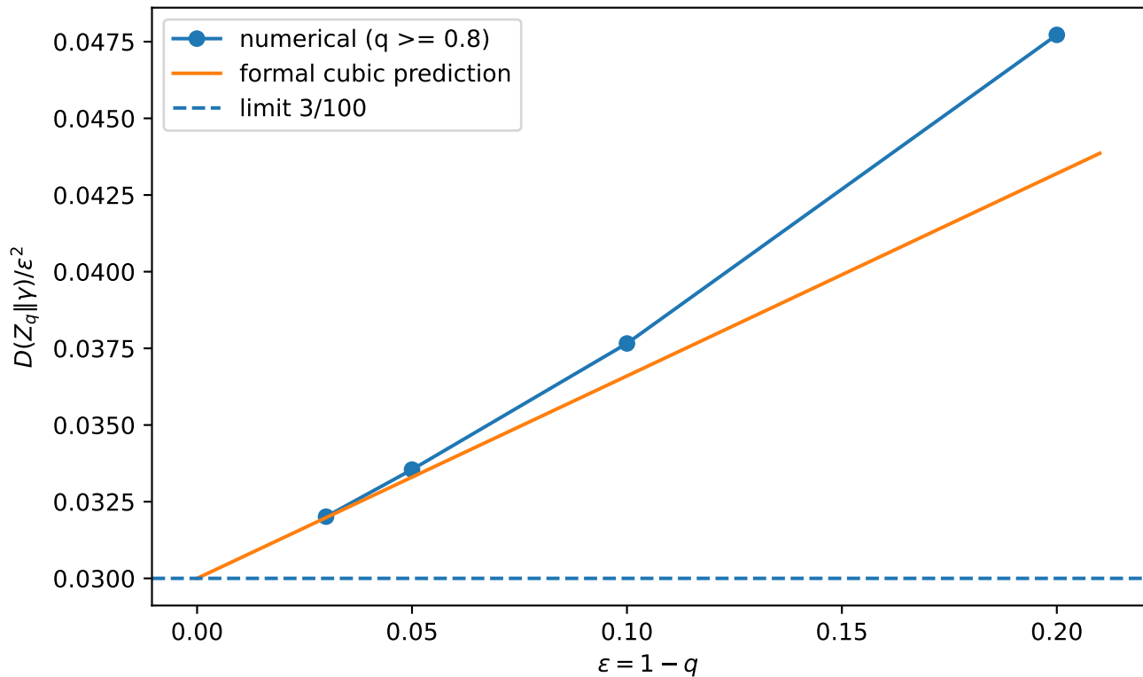
Entropic Gaussian limit of the geometric-uniform law
