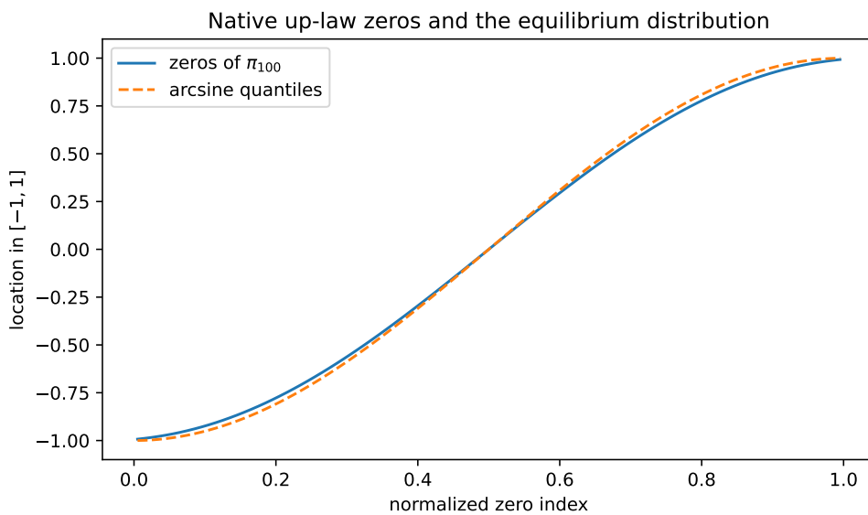
Figure 1: Zeros of \pi_{100} , computed as eigenvalues of the finite Jacobi matrix, against the arcsine quantiles. This is a numerical illustration of equation (5.7), not an additional proof.
