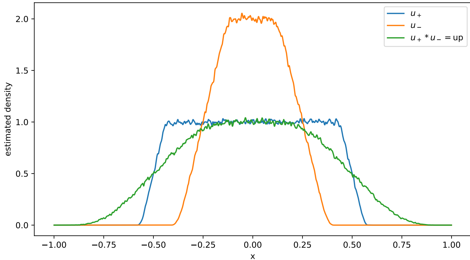
Thue-Morse scale factors and their Rvachev convolution
