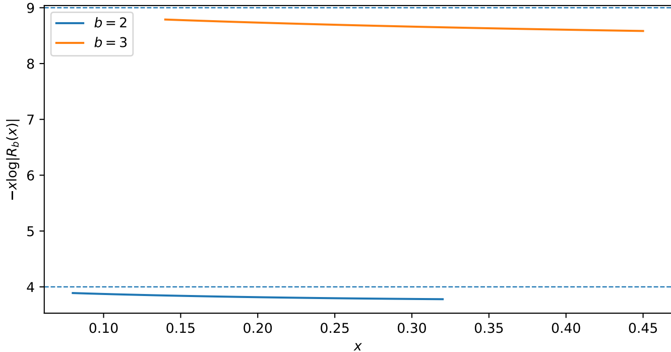
Beyond-all-orders remainder: first scale e^{-b^2/x}
