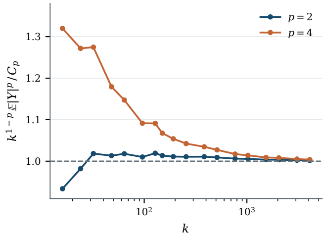
Scaled moments approach their constants
