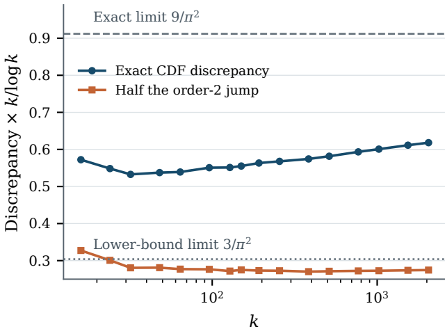
The logarithmic discrepancy scale
