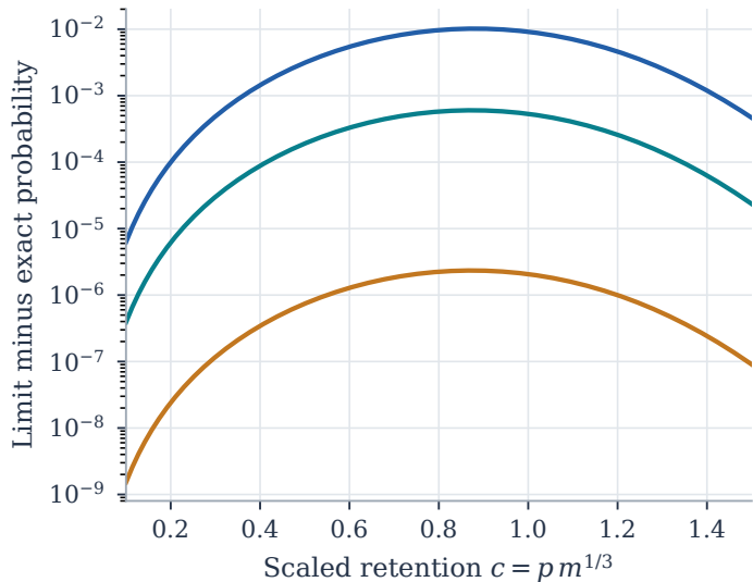
(b) Difference from the limit
