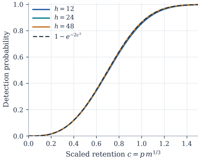
(a) Exact Bernoulli detection
