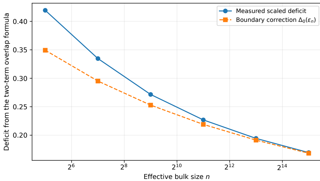
Figure 2: The measured scaled overlap deficit and the independently computed compact correction \Delta_0(\varepsilon_n) . Their difference is consistent with the O((\log n)^3/n) error in (2.13). This plot diagnoses a slow boundary effect; it is not a proof of the asymptotic bound.
