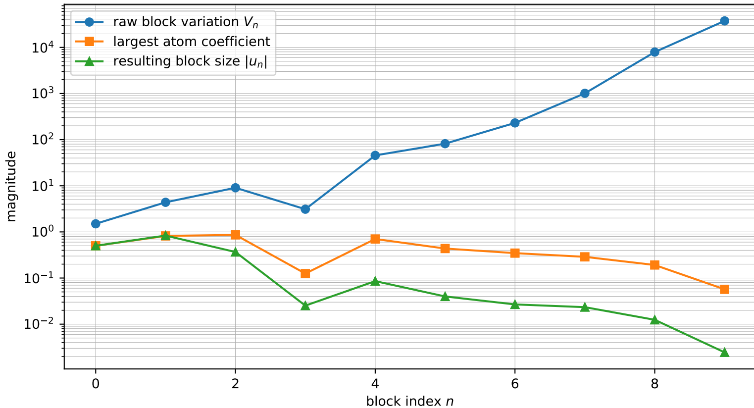
Internal cancellation in the exact Legendre--up blocks
