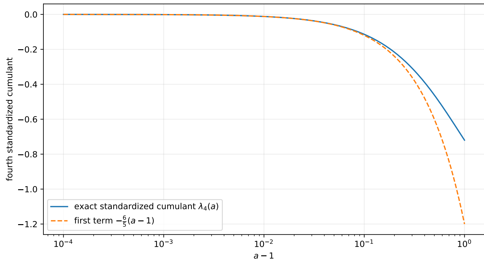
Gaussian limit as the base decreases to one
